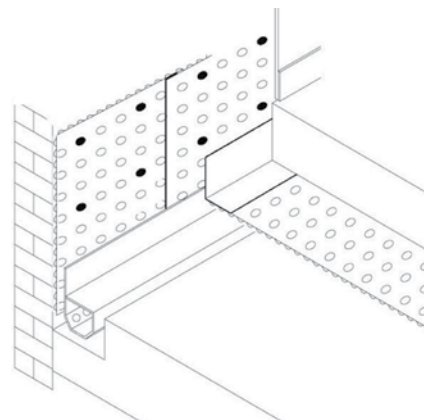
Typical basement conversion detail using Baseline 8 membrane on floors and walls, butyl tape to seal joints and Aqua-Channel for drainage.
