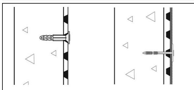
Figure 2 Membrane Plug and Mesh Membrane Plug
