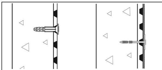
Figure 2 Membrane Plug and Mesh Membrane Plug
