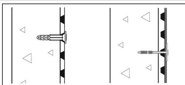
Figure 2 Membrane Plug and Mesh Membrane Plug
